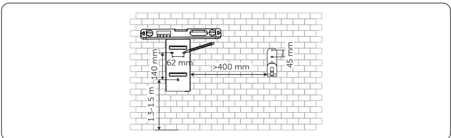
Figure 6-7 Mark the holes
