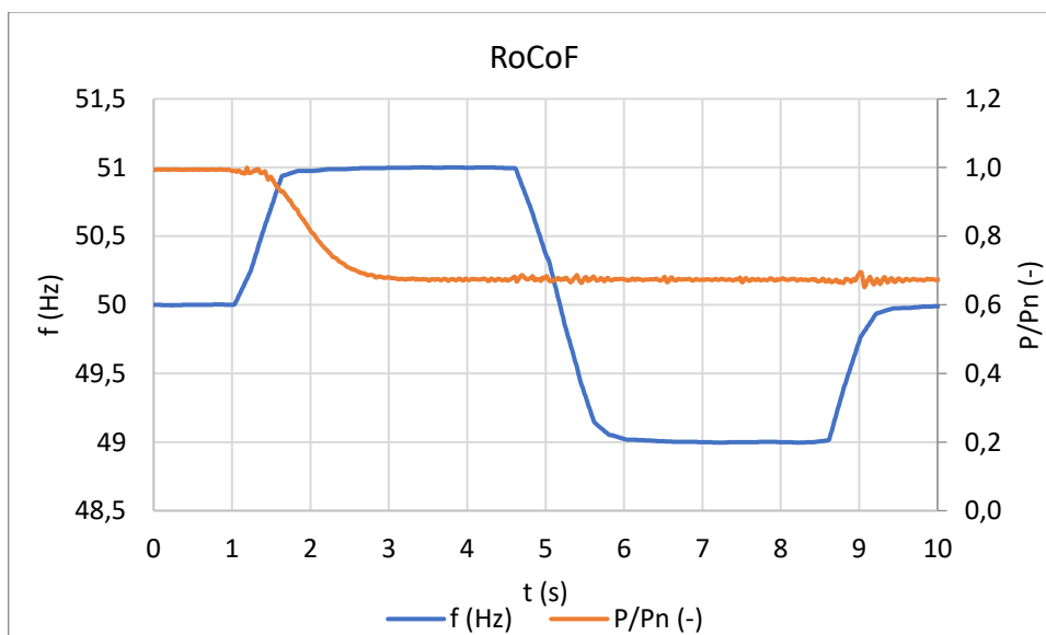
Obr.2.1: RoCoF
